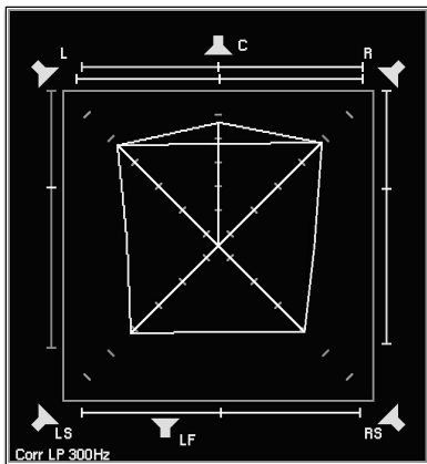
4. Surround signal with some Center presence (roof). A support microphone would be too dominant. A dialog in relation to music would be too quiet. The width of the PSI lines of the C channel is a sign of coherent signal parts in L and/or R (crosstalk).
