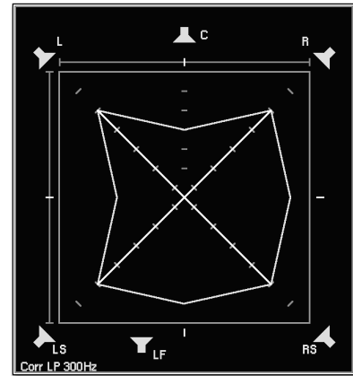
3. Same as on the left but with the phase of the left channel rotated through 180^\circ . In the channel pairs L - R and L - LS each the correlation is r = -1 , there are no phantom sound sources locatable.
