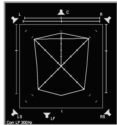
6. The widely outward broken TVI line between LS and RS, no spreading of the PSI line and the correlation level r = +1 in the lower phase meter indicate that an identical mono signal is applied in both surround channels.
