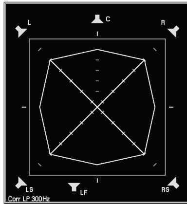
2. Identical sine wave signal with same level in the channels L, R, LS, RS. The correlation is r = +1 (outward broken TVI lines), the phantom sound sources (PSI) are in the middle, similar to a mono signal.
